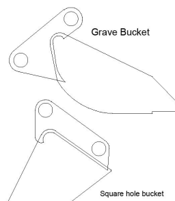
Grave and square hole digging buckets for 1 to 6 ton machines
